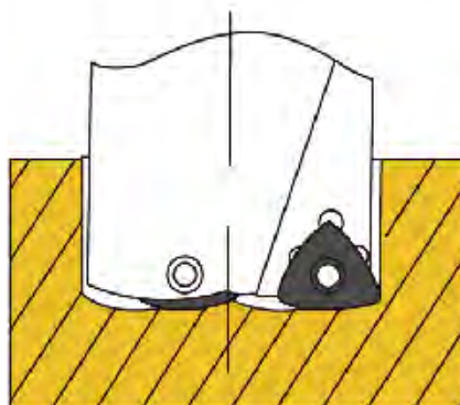
WC Insert Shallow hole drill
